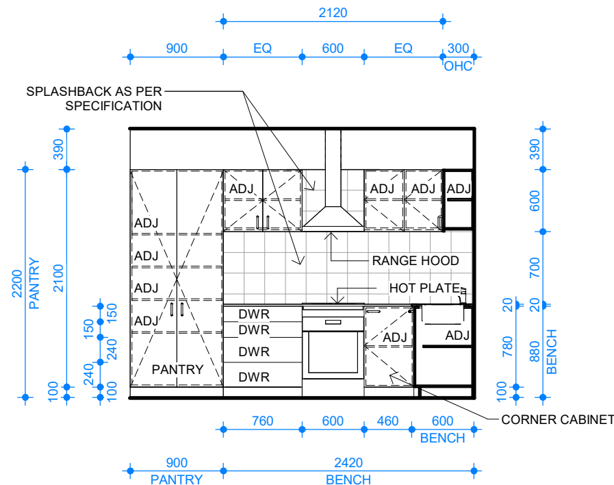
1 KITCHEN ELEVATION
