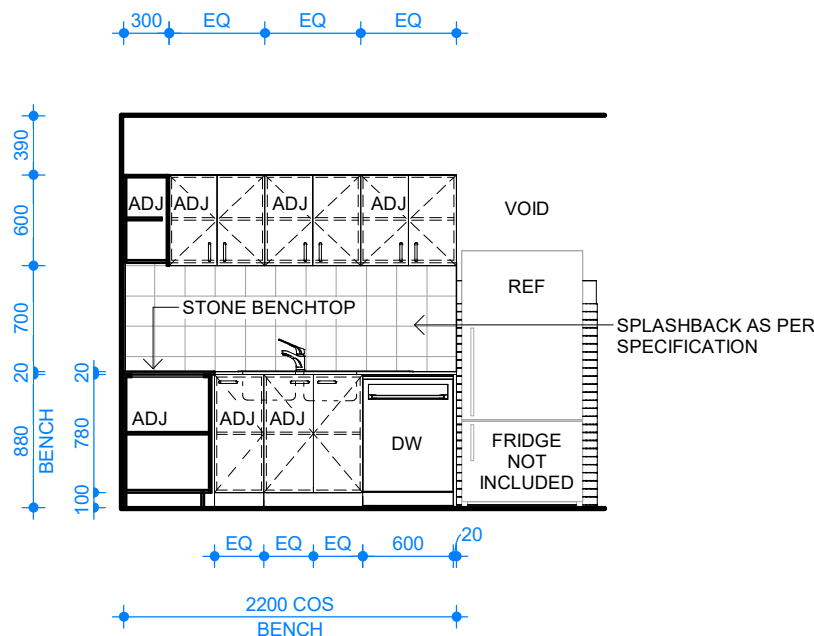
2 KITCHEN ELEVATION
