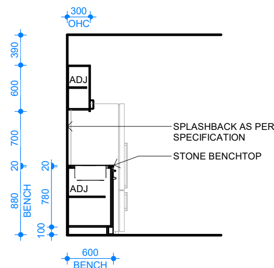
3 KITCHEN ELEVATION
