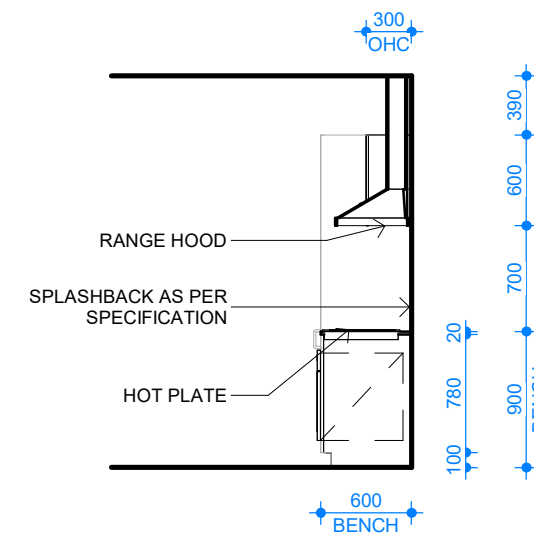
4 KITCHEN ELEVATION
